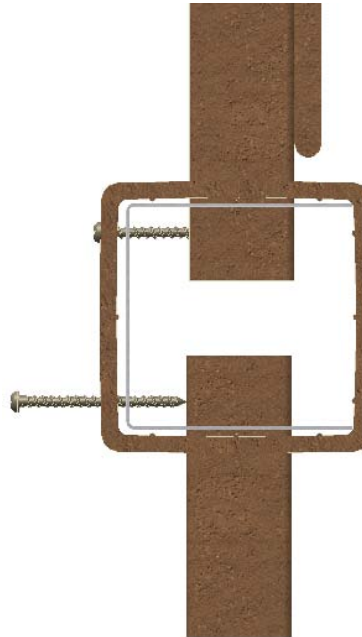
Screw secures sleeve, steel insert and backer rail without pilot holes
