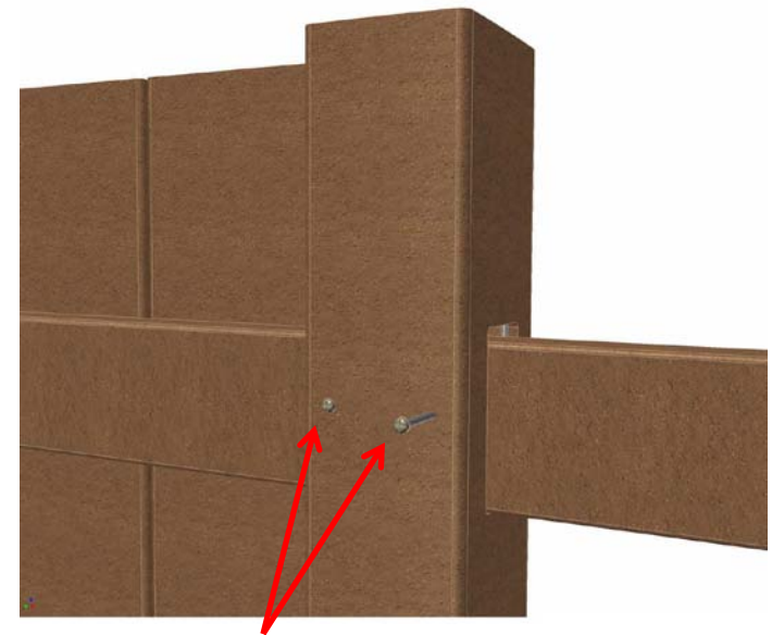
Line Post uses 2 screws per post
